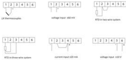
Fig. 2 Connection to measuring inputs.
