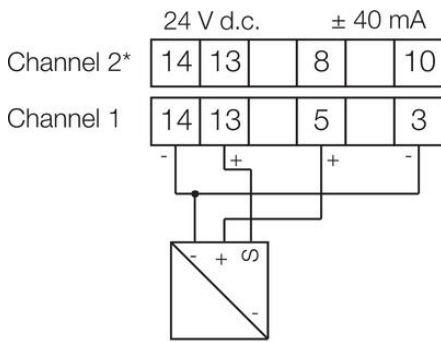
3-wire object transducer
