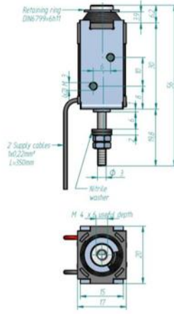
Solenoid locked
