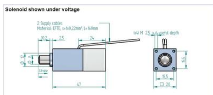
Solenoid shown under voltage
