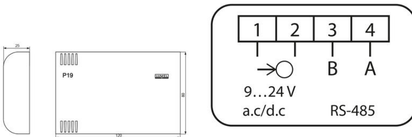
Connection diagram
