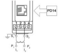
d) indirect measurement of current by means of current transformer
