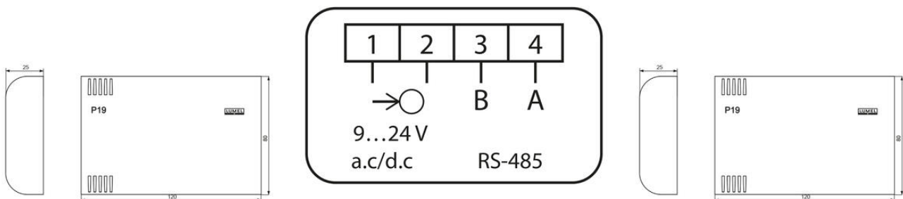
Connection diagram
