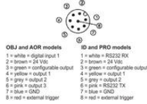
M12 8-pole (power supply and I/O)
