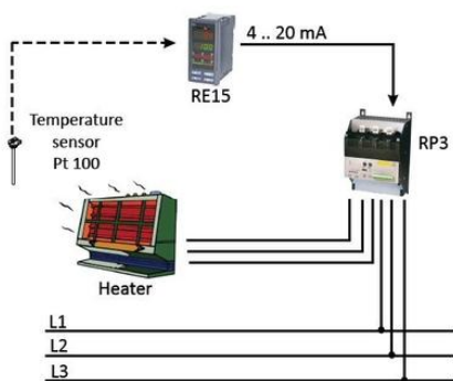
Control of a three-phase heater.
