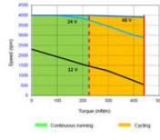
Speed-torque and current-torque curves
