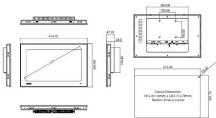
Panel Cut-out Dimension: 412.40 x 261.70 mm (16.24" x 10.30")
