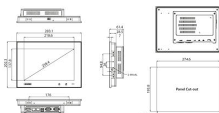
TPC-1051WP Panel Cut-out Dimensions: 274.6 x 193.8 mm
