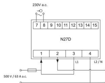
Connection diagram
