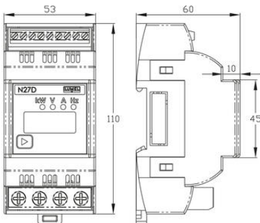
External dimensions
