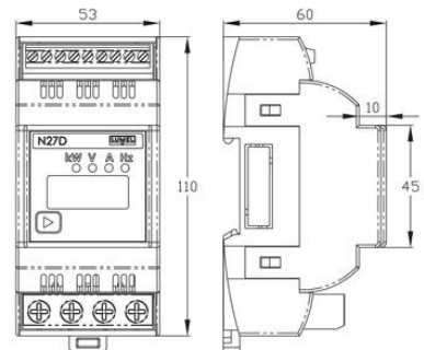
External dimensions
