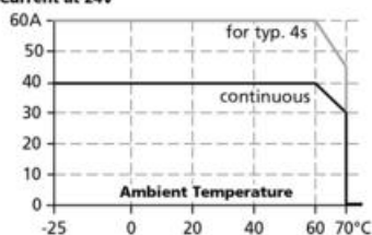
Allowed Output Current at 24V
