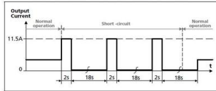
Fig. 6-3 Short-circuit on output, Hiccup SM mode, typ.
