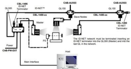
ID-NET™ Synchronized Network - Matrix 400™ Master with QL150 + Matrix 400™ Slaves with QL150
